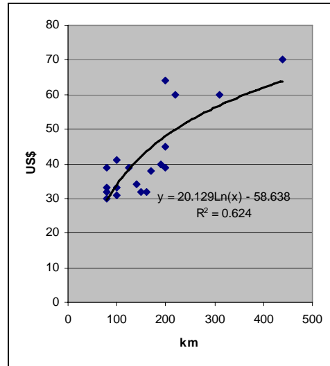
Figure 3: Trucking costs per m 3 of timber, Mozambique, 2004
