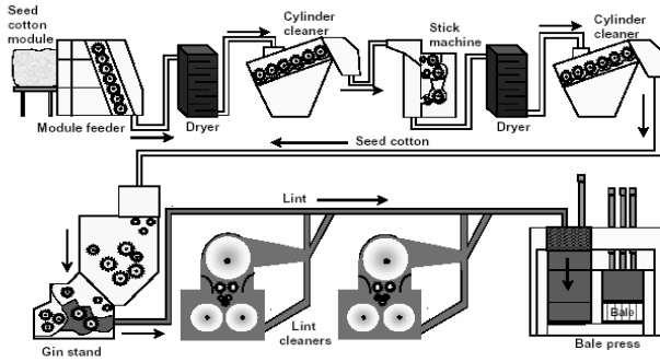
Diagram 5: Representative cross-section of the typical ginning process
